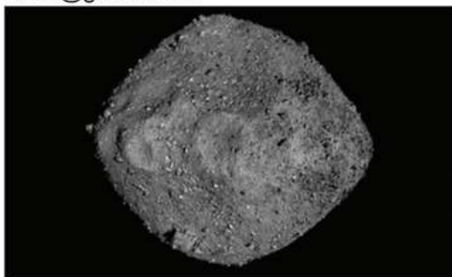
This mosaic of Bennu was created using observations made by NASA's OSIRIS-Rex spacecraft that was in close proximity to the asteroid for over two years. Credit: NASA/Goddard/University of Arizona
